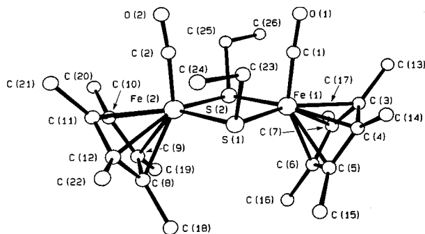
Fig. 4 Perspective view of the [\text{Fe}_2(\eta\text{-C}_5\text{Me}_5)_2(\mu\text{-SEt})_2(\text{CO})_2]^+ cation in complex 2
