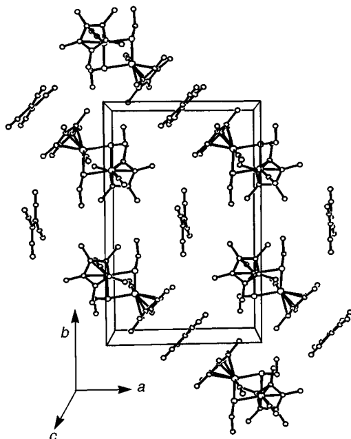
Fig. 5 Packing of [\text{Fe}_2(\eta\text{-C}_5\text{Me}_5)_2(\mu\text{-SEt})_2(\text{CO})_2]^+ cations and \text{tcne}^- anions in crystals of 2
