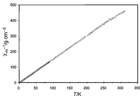
Fig. 6 Linearised plot of \chi_\text{m}^{-1} against temperature for [\text{Fe}_2(\eta\text{-C}_5\text{Me}_5)_2(\mu\text{-SEt})_2(\text{CO})_2][\text{tcne}] 2
