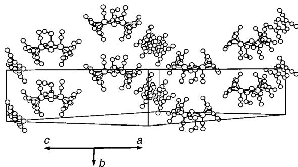
Fig. 2 Packing of [\text{Fe}_2(\eta\text{-C}_5\text{Me}_5)_2(\mu\text{-SEt})_2(\text{CO})_2]^+ cations and (\text{tcnq})_2^{2-} dimers in crystals of complex 1
